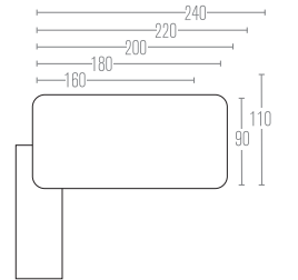
U TOO W:90-110 CM 2 LEG DESKS | 2 AYAK MASALAR | SCRIVANIE A 2 GAMBE | 2 BEIN-SCHREIBTISCHE
